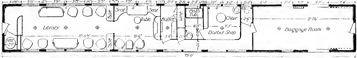
Fig. 175. SECTIONAL PLAN OF COMBINATION BAGGAGE, BARBER SHOP, BATH ROOM AND LIBRARY CAR, COLUMBUS. (Interior view is shown in Fig. 132.)
